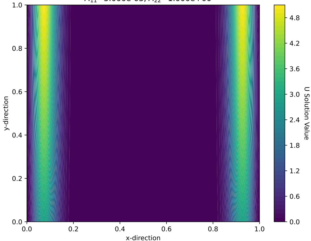
RBF-FD Approximate Solution (Contour): A_{11}=5.000\text{e-}03 , A_{22}=1.000\text{e+}00
